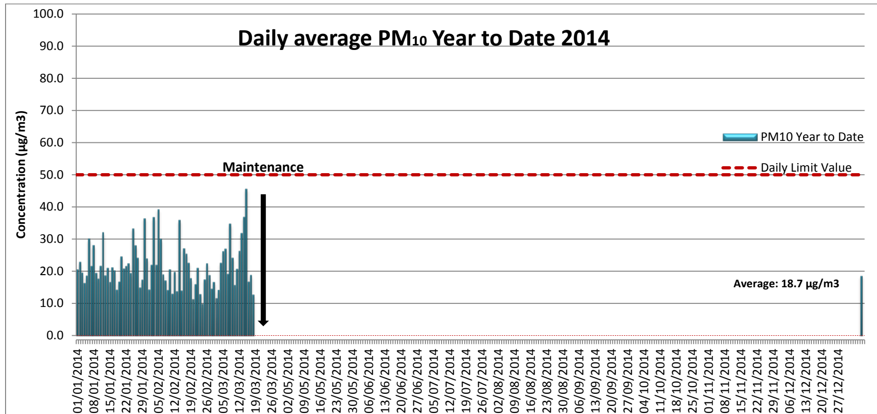
Figure 5: Daily Average PM 10 2014
