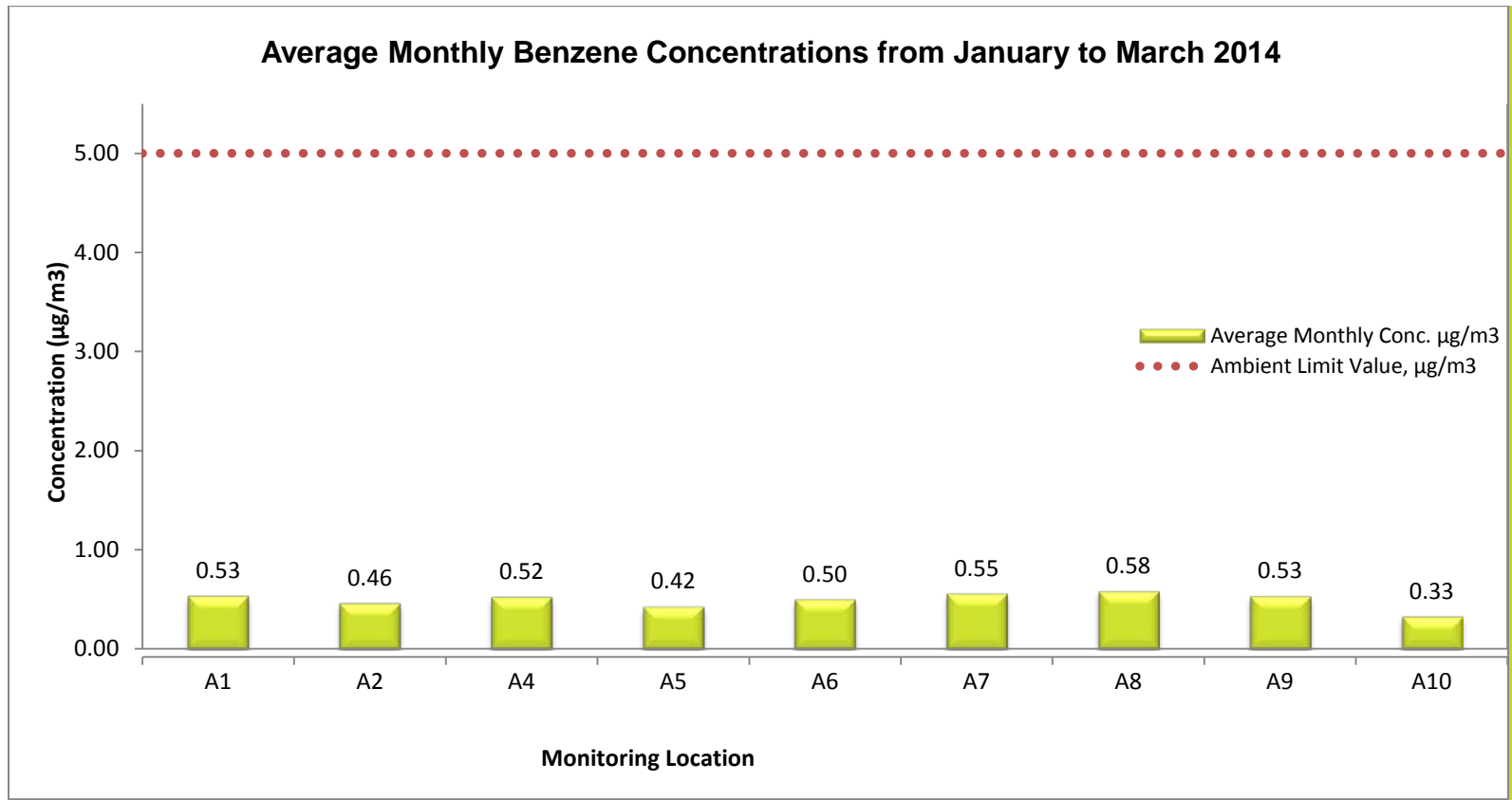
Figure 3: Average Monthly Benzene (C 6 H 6 ) Concentrations 2014 Q1
