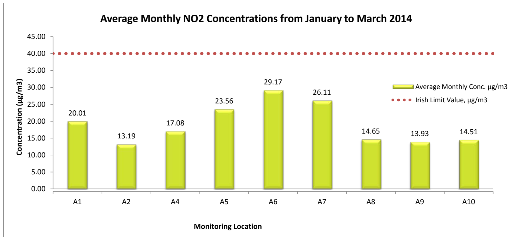
Figure 2: Average Monthly NO 2 Concentrations 2014 Q1
