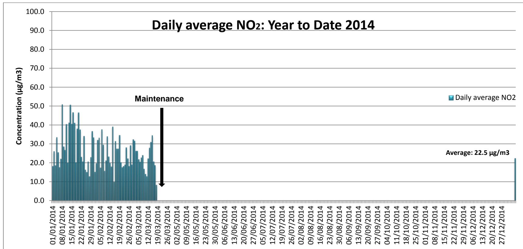
Figure 4: Daily Average NO 2 2014
