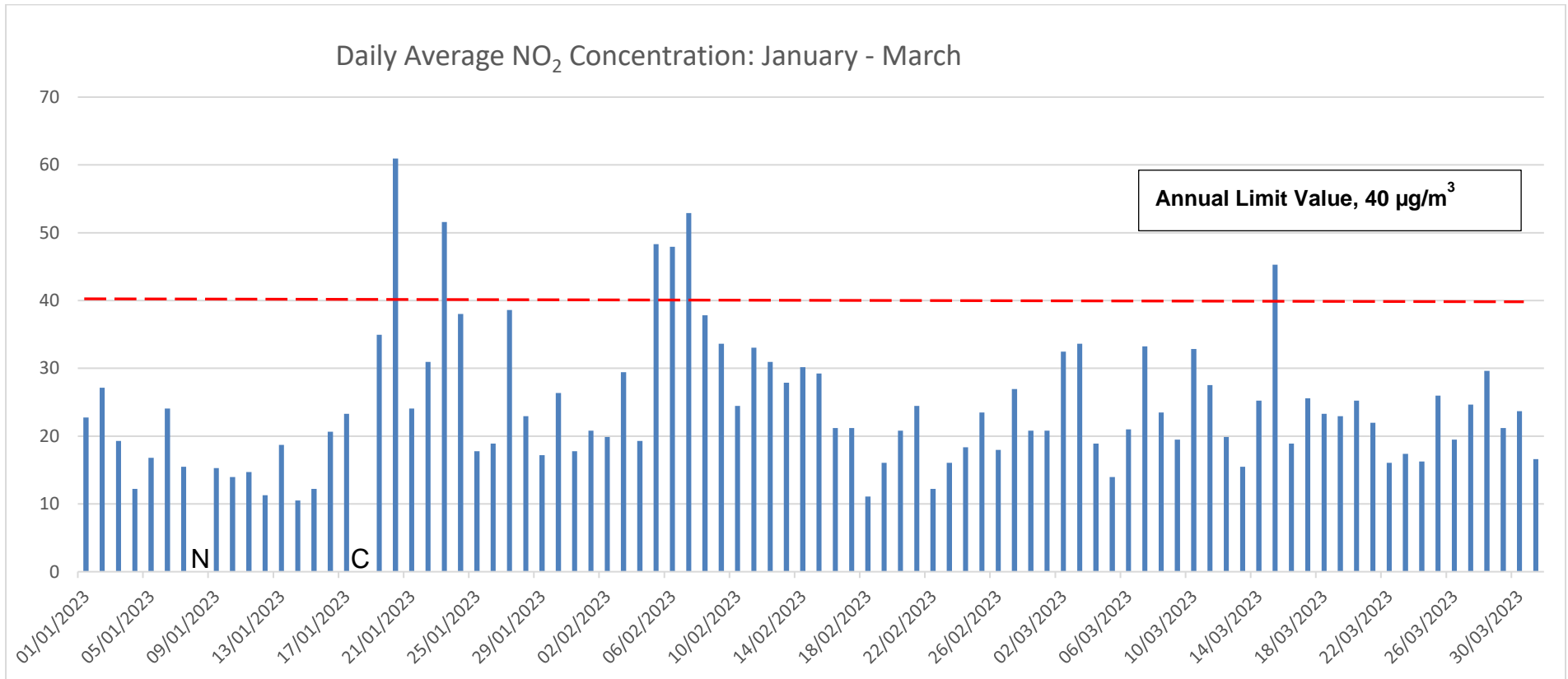
Figure 4 Daily Average NO 2 Q1 2023
