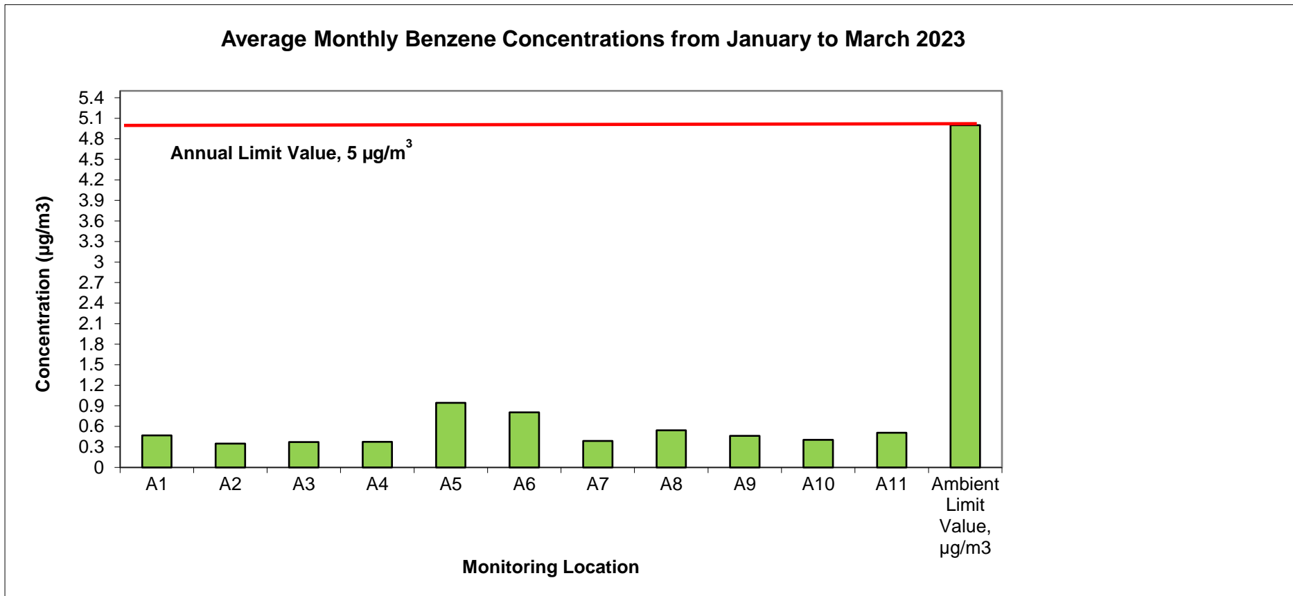
Figure 3 Average Monthly Benzene (C 6 H 6 ) Concentrations Q1 2023
