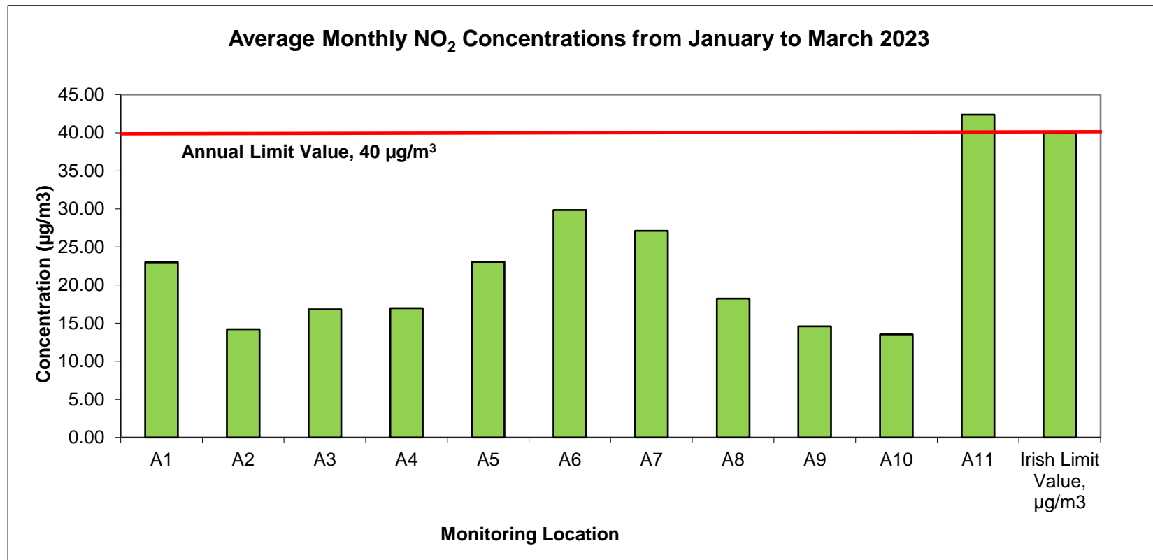
Figure 2 Average Monthly NO 2 Concentrations Q1 2023
