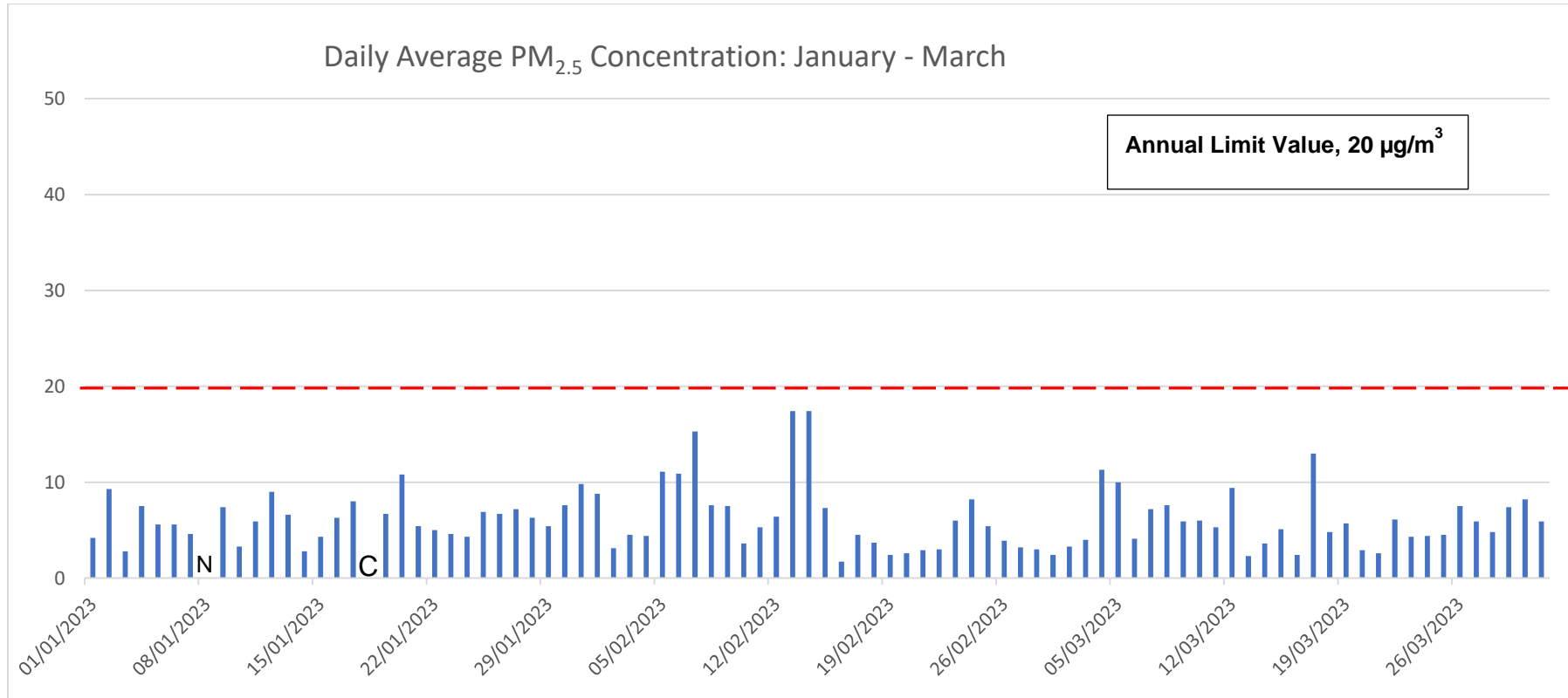
Figure 6 Daily Average PM 2.5 Q1 2023
