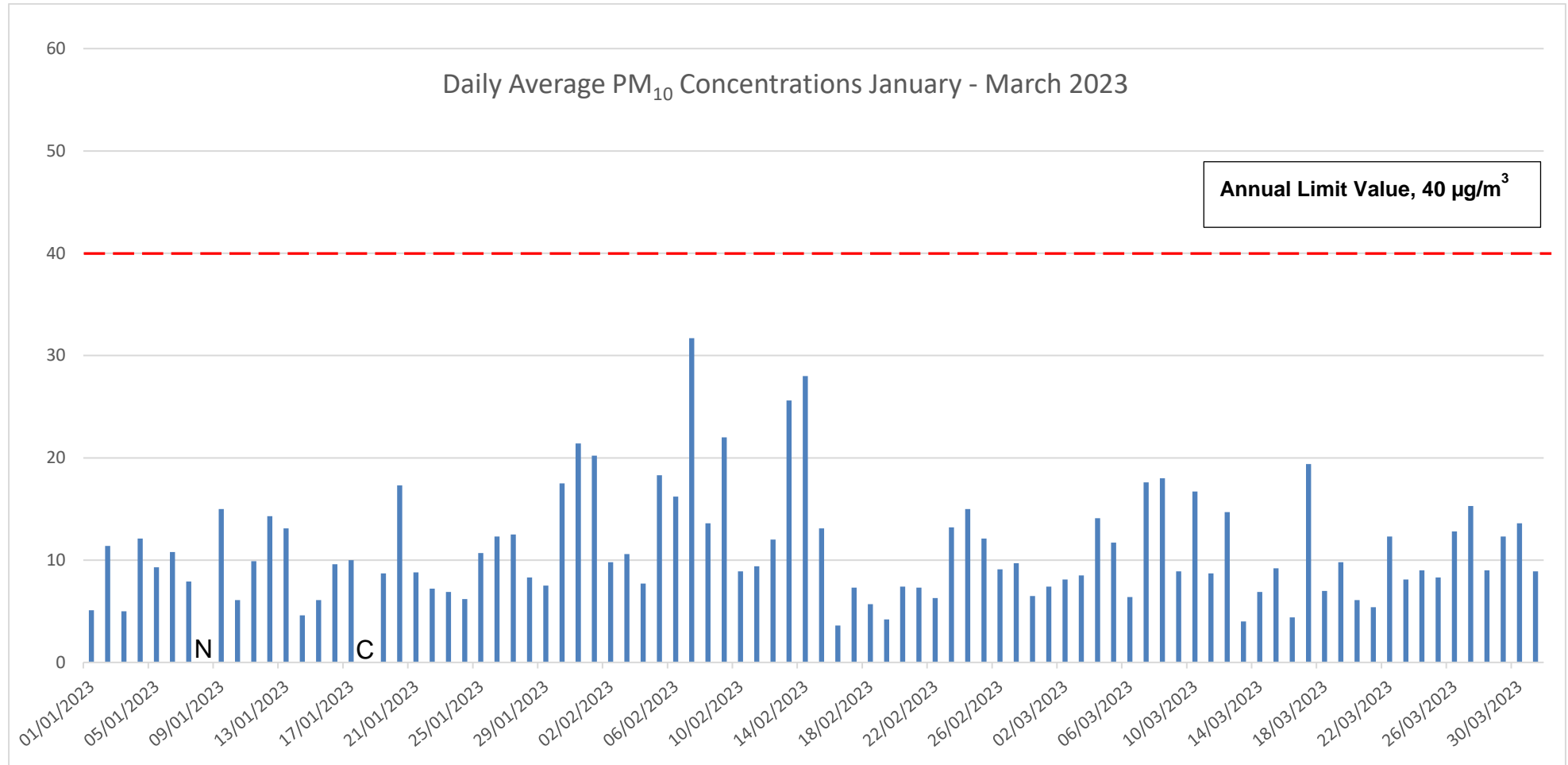
Figure 5 Daily Average PM 10 Q1 2023
